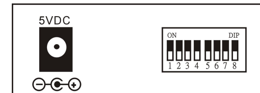
Fig. 3 Rear Panel
