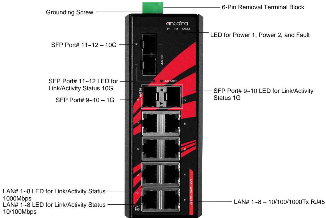
Figure 2.2 - The Front Panel of LNX-1204G-10G-SFP
