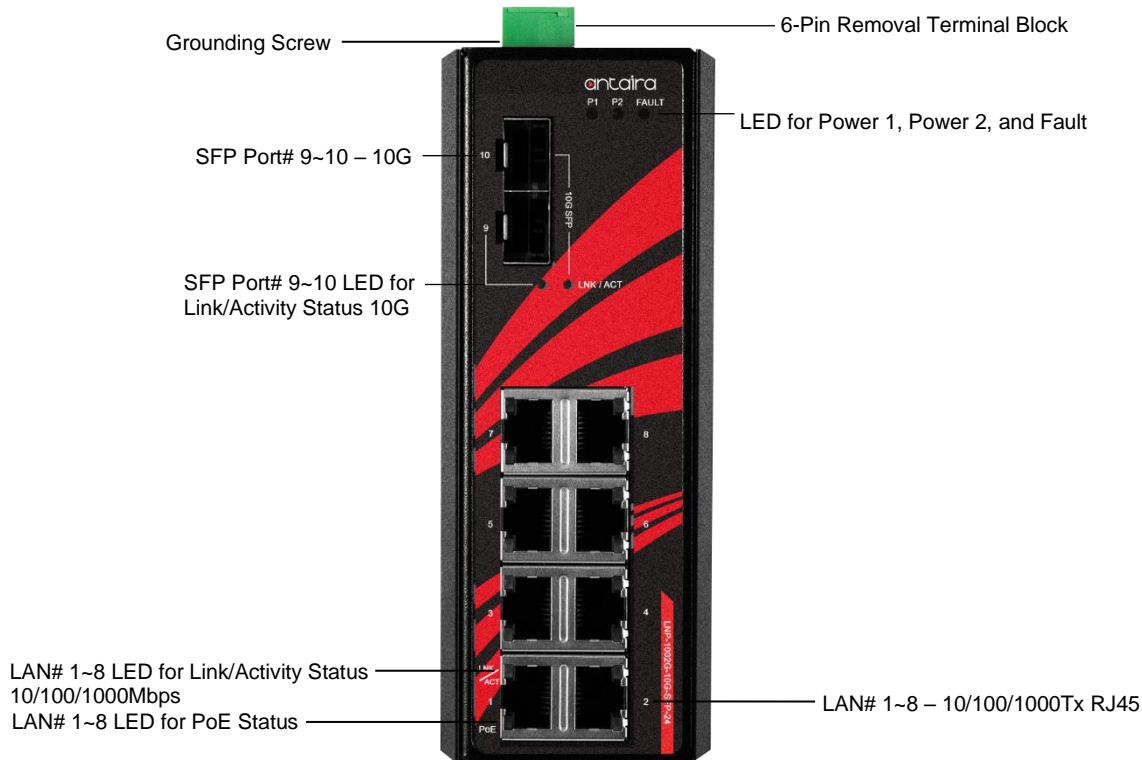
Figure 2.2 - The Front Panel of LNP-1002G-10G-SFP-24
