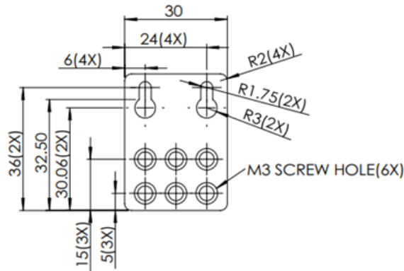
Figure 3.5 - Wall Mounting Bracket Dimensions
