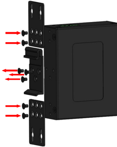
Figure 3.4 - Remove DIN-Rail bracket from the Switch and place the wall mounting brackets
