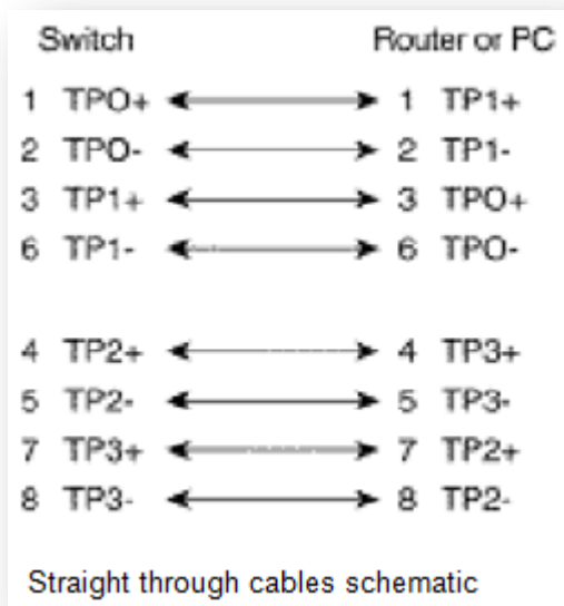
Figure 2.7 - Straight-Through Cables Schematic
