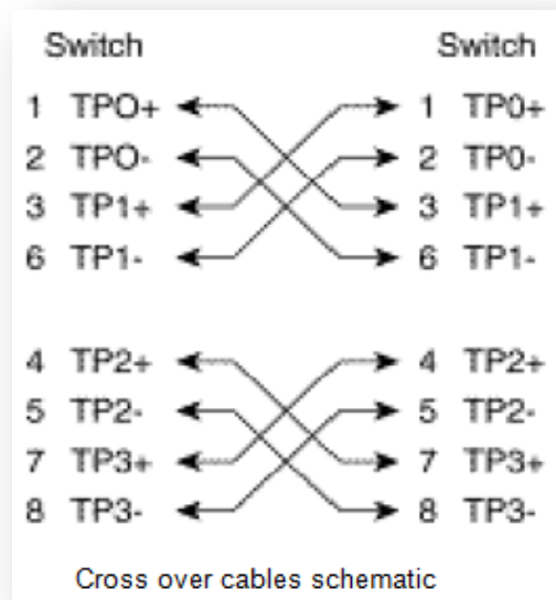
Figure 2.8 - Crossover Cables Schematic
