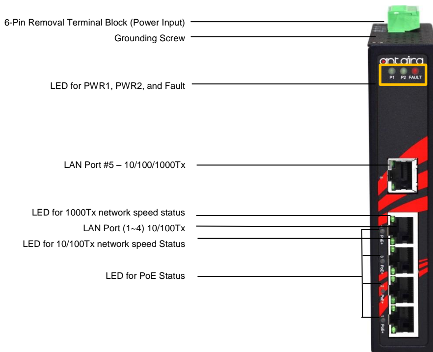
Figure 2.2 Front Panel of the LNP-0500G Series
